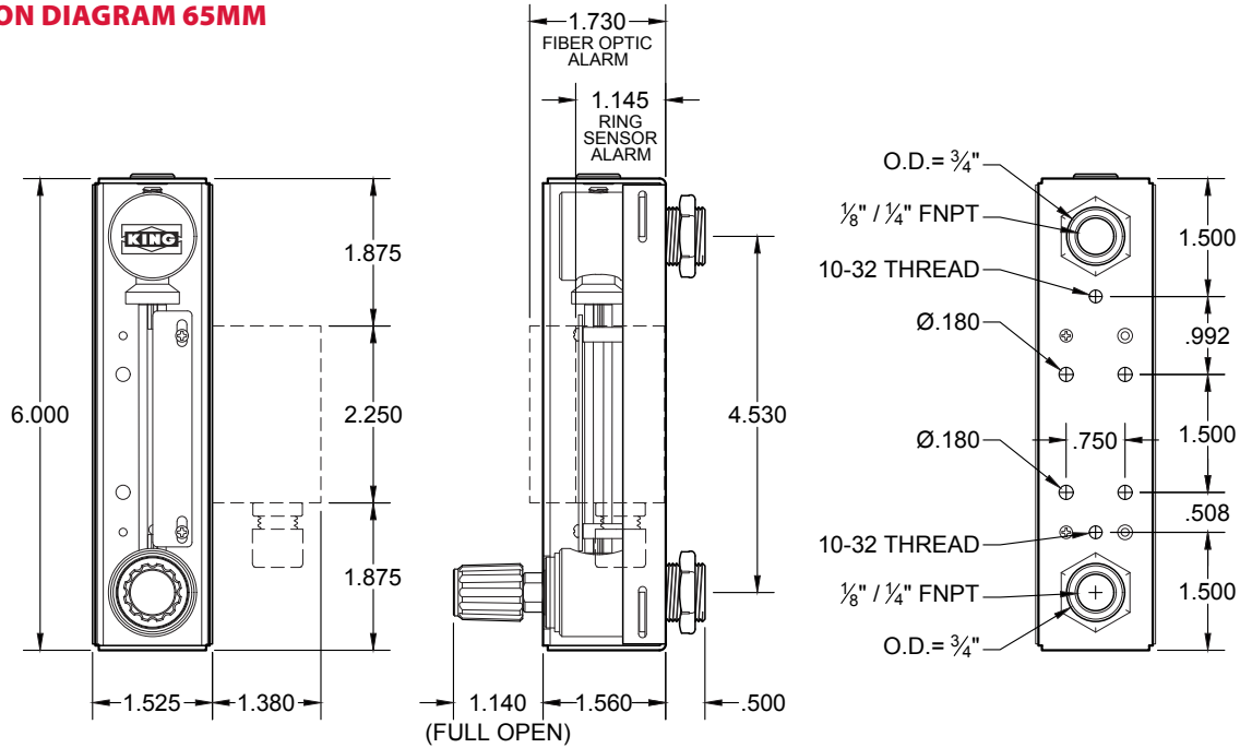
DIMENSION DIAGRAM 65MM
